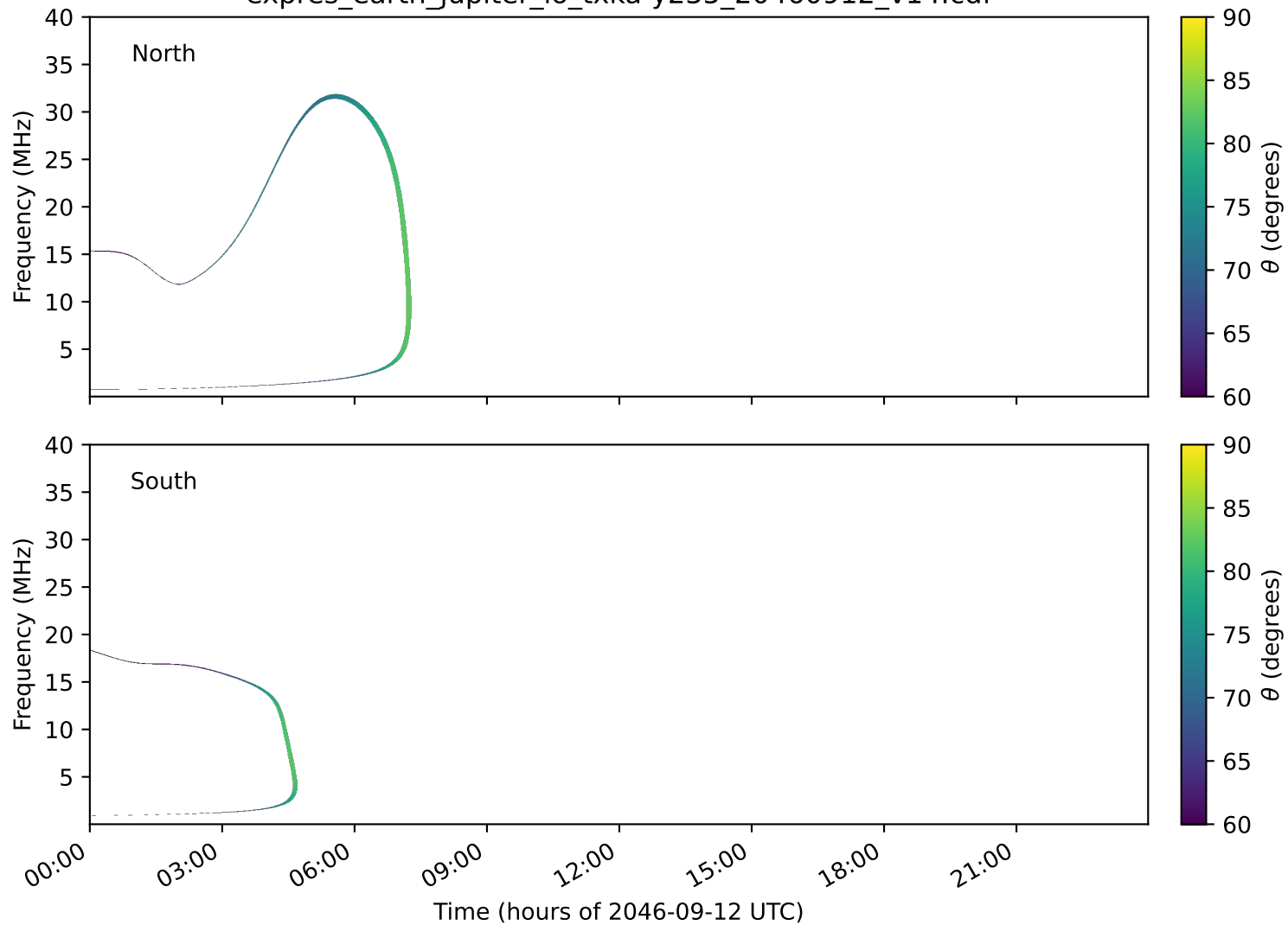
expres_earth_jupiter_io_txka-y235_20460912_v14.cdf
