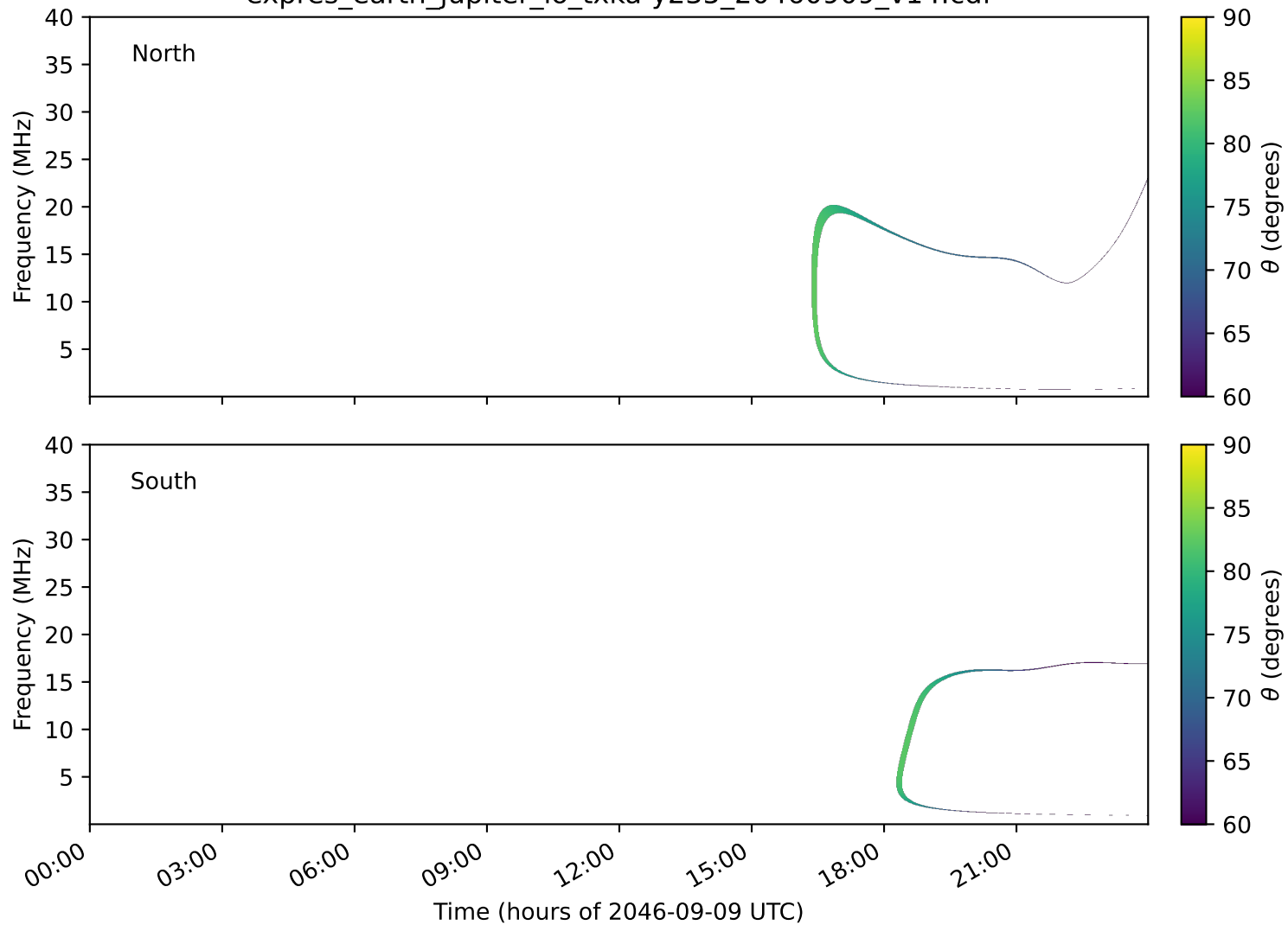
expres_earth_jupiter_io_txka-y235_20460909_v14.cdf
