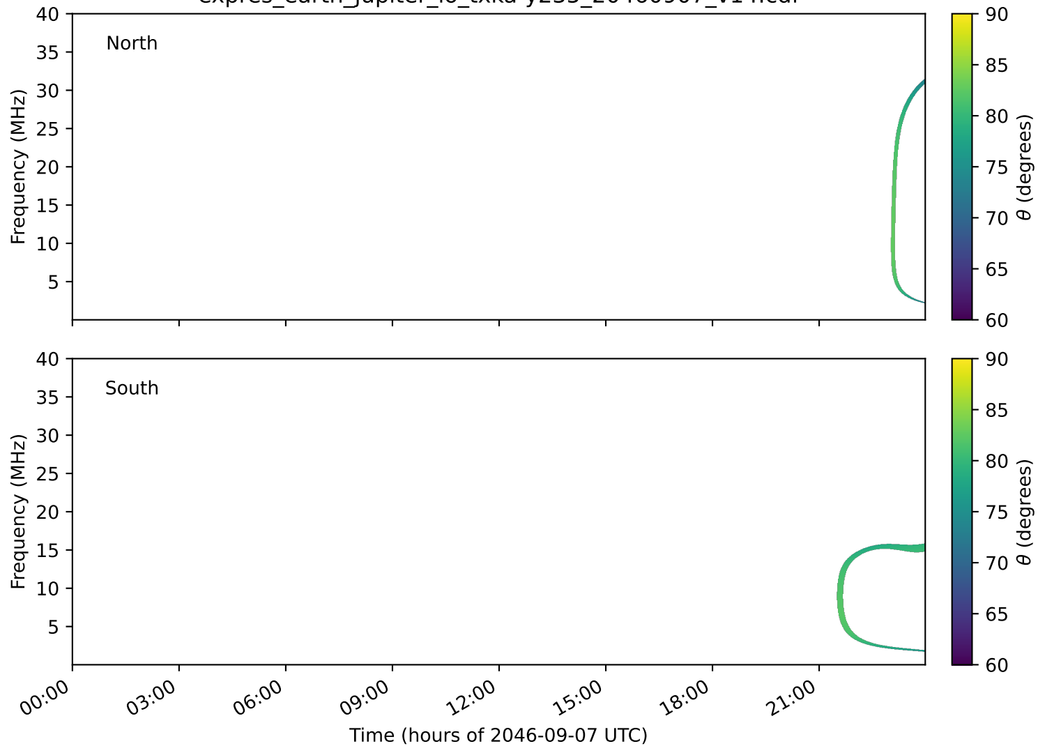
expres_earth_jupiter_io_txka-y235_20460907_v14.cdf
