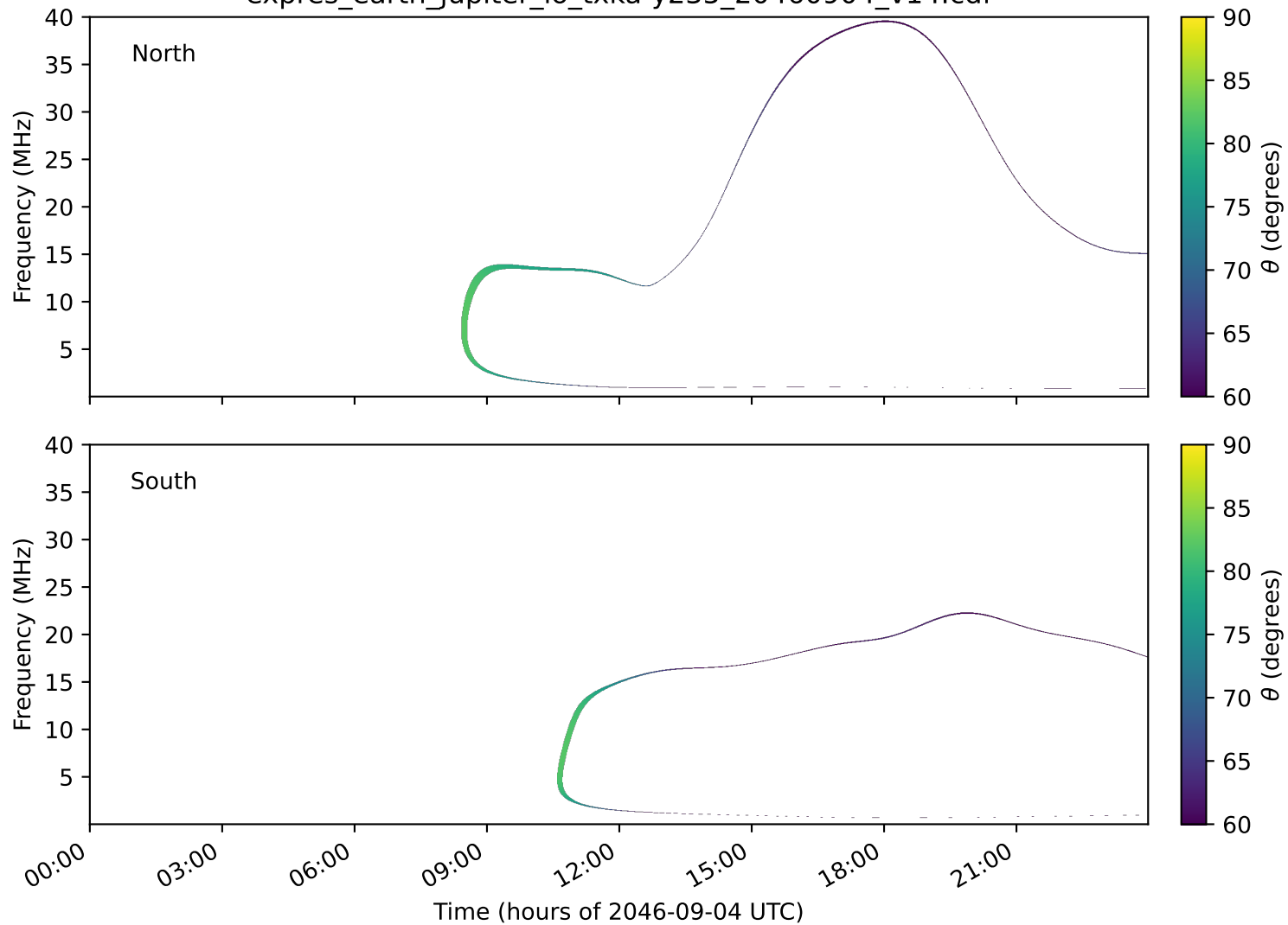
expres_earth_jupiter_io_txka-y235_20460904_v14.cdf
