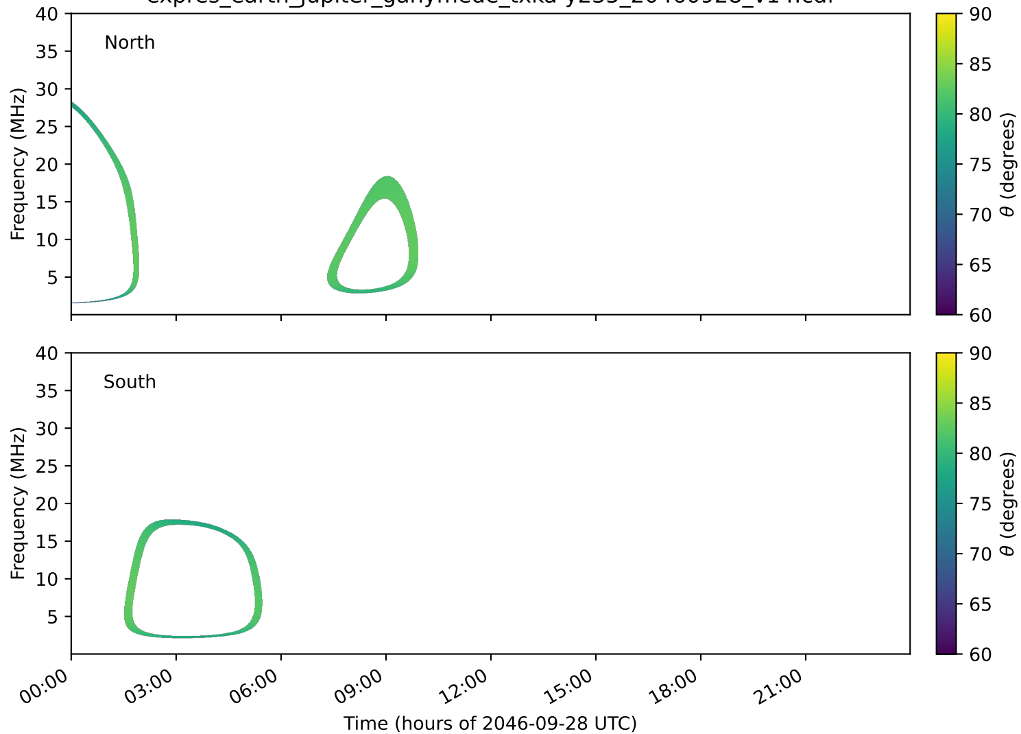
expres_earth_jupiter_ganymede_txka-y235_20460928_v14.cdf
