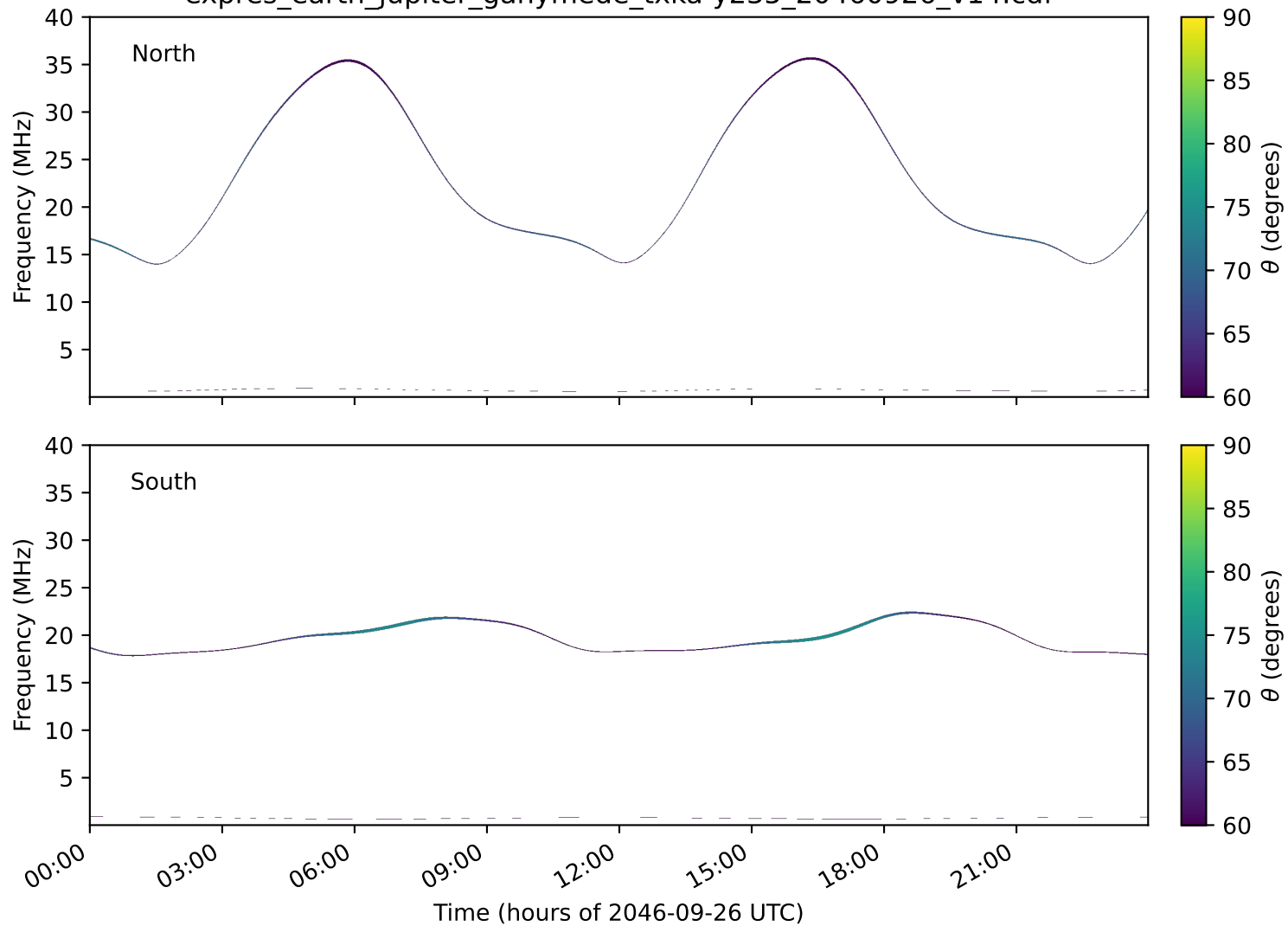
expres_earth_jupiter_ganymede_txka-y235_20460926_v14.cdf
