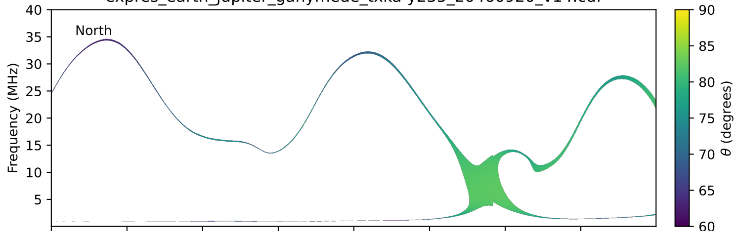
expres_earth_jupiter_ganymede_txka-y235_20460920_v14.cdf
