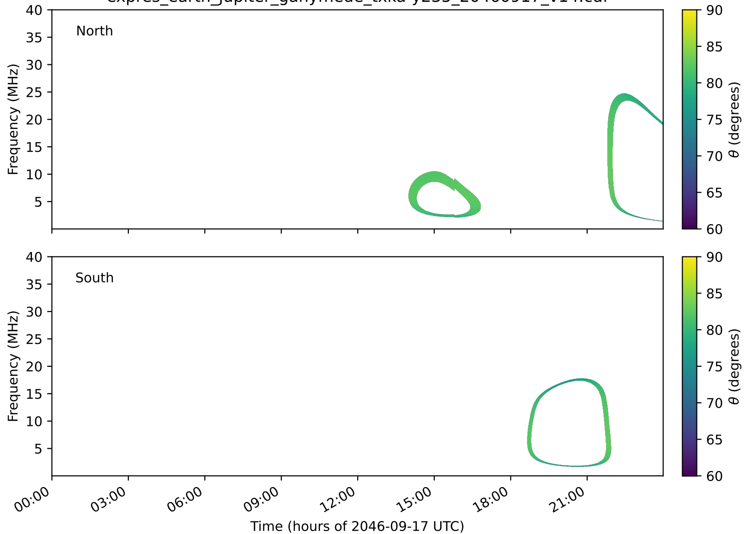
expres_earth_jupiter_ganymede_txka-y235_20460917_v14.cdf
