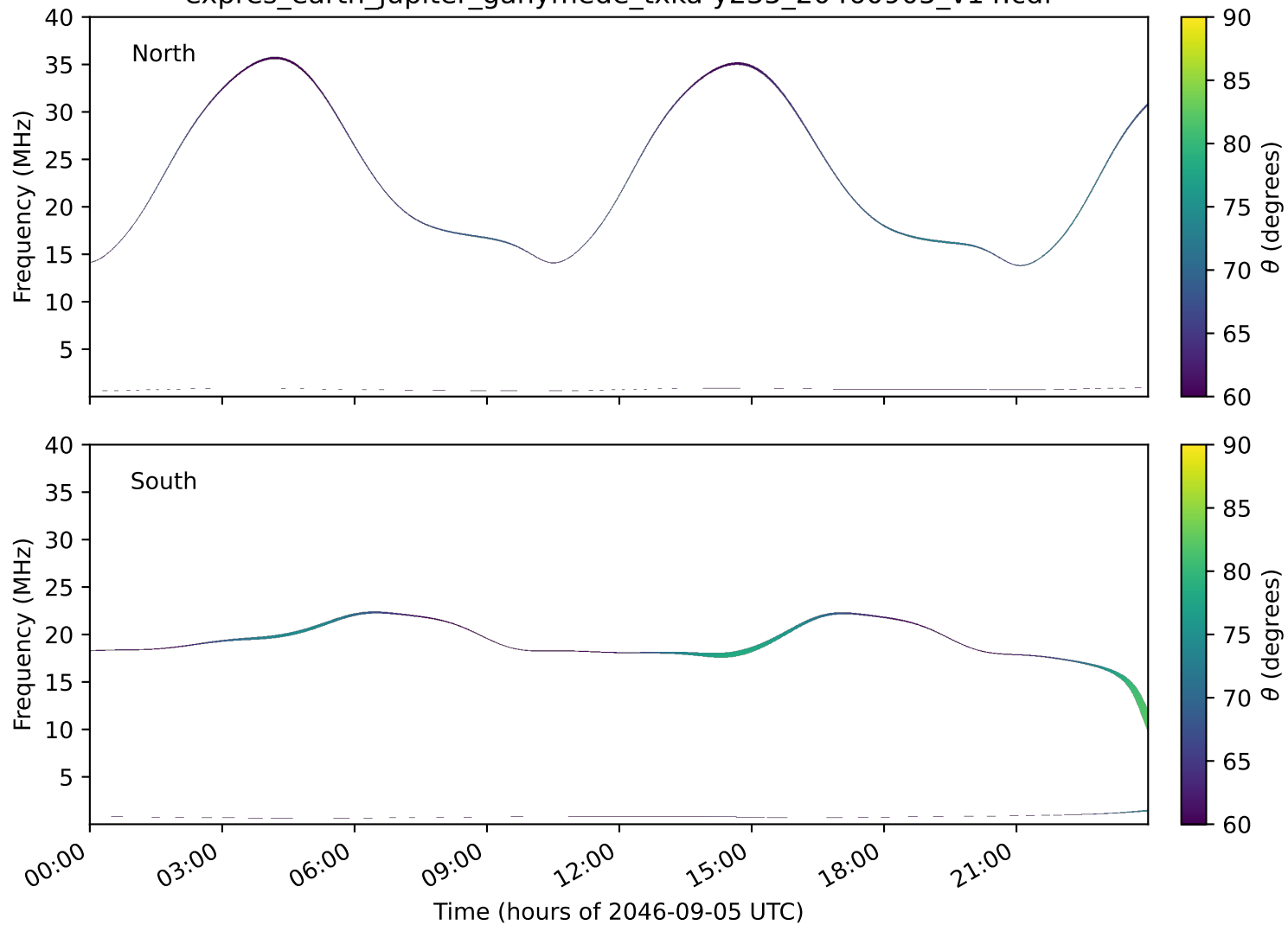
expres_earth_jupiter_ganymede_txka-y235_20460905_v14.cdf
