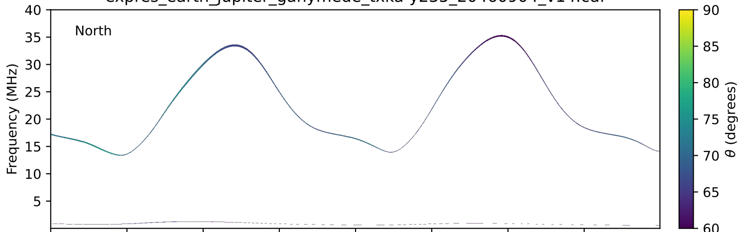
expres_earth_jupiter_ganymede_txka-y235_20460904_v14.cdf
