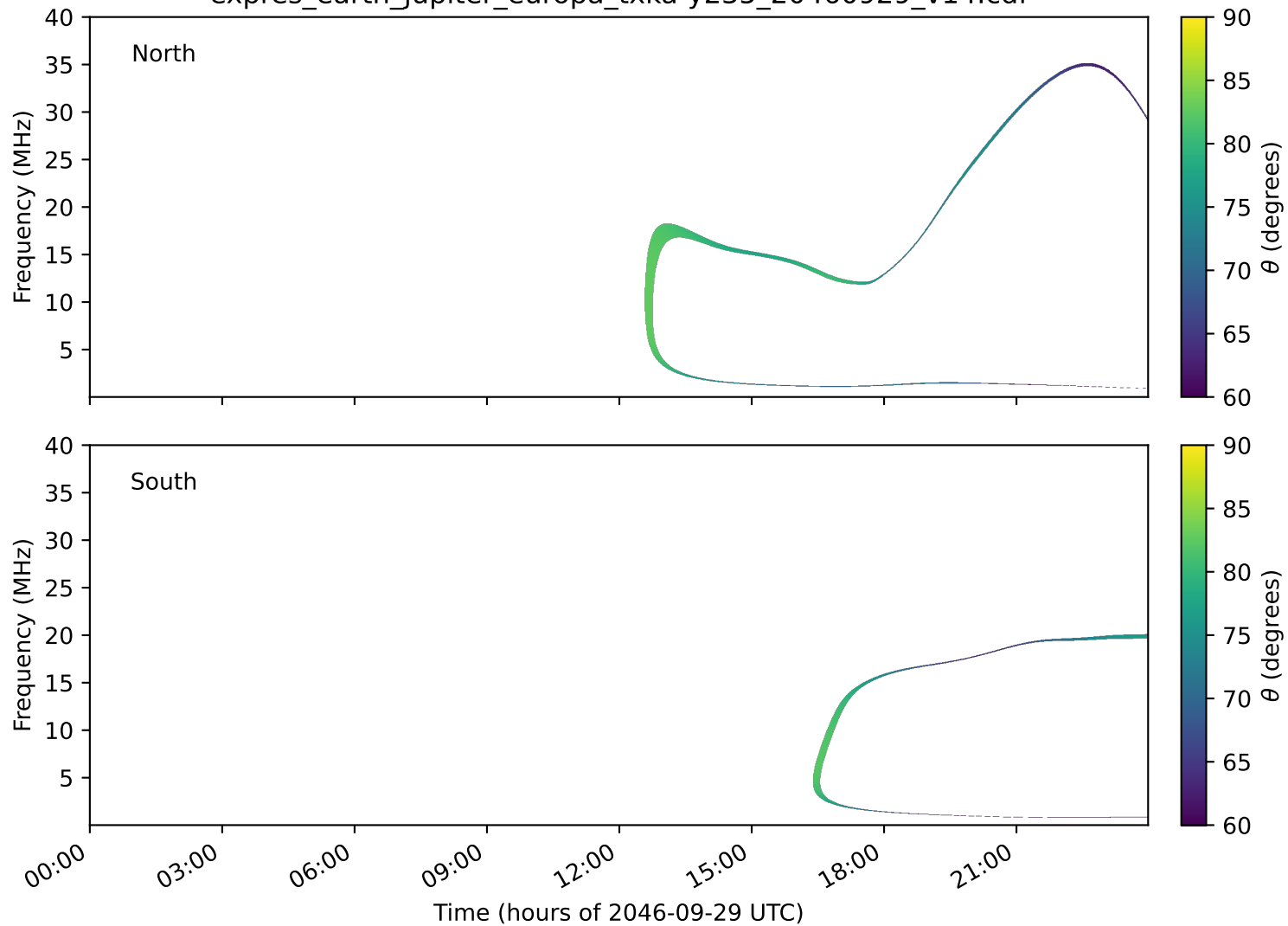
expres_earth_jupiter_europa_txka-y235_20460929_v14.cdf
