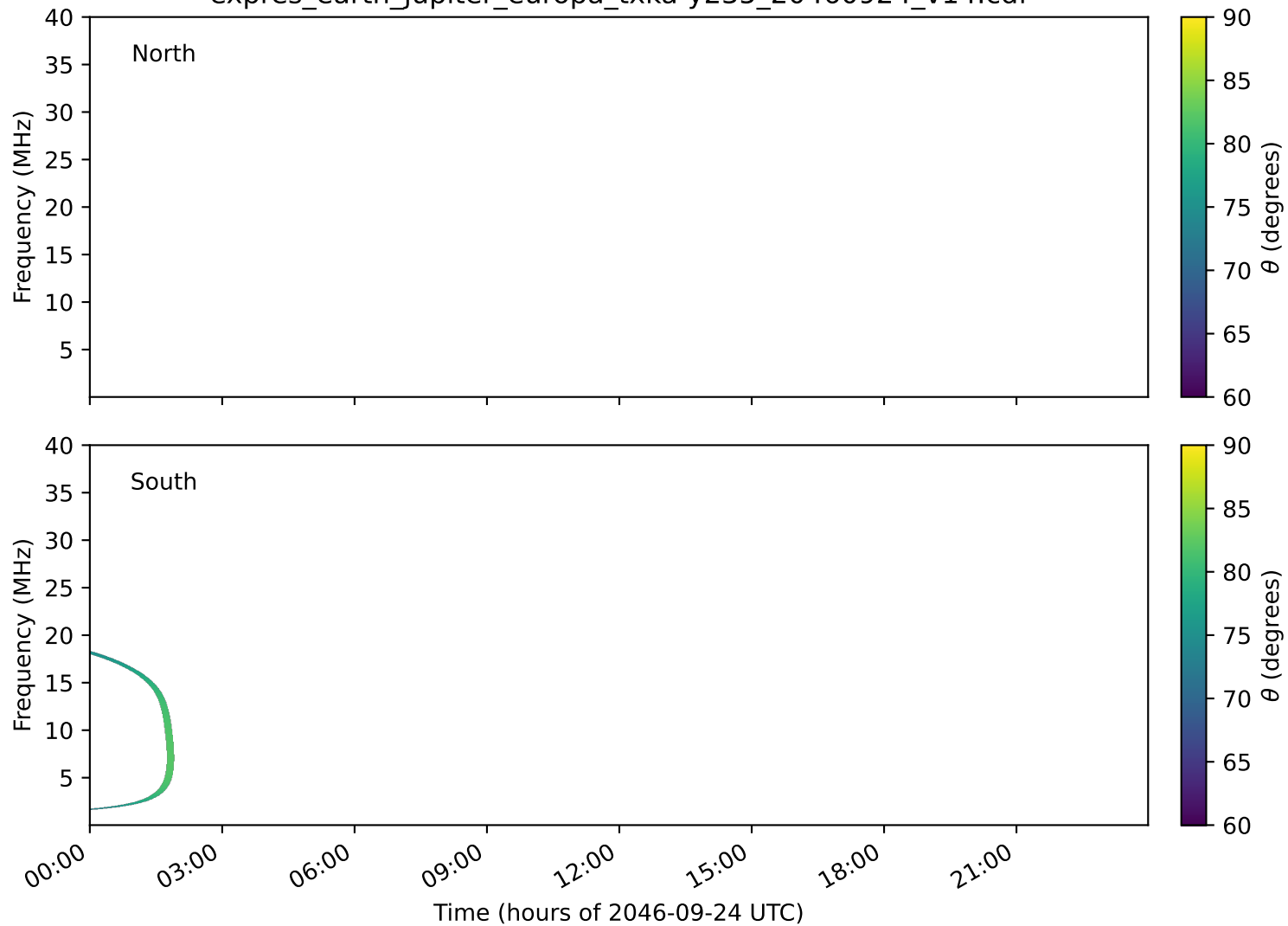
expres_earth_jupiter_europa_txka-y235_20460924_v14.cdf
