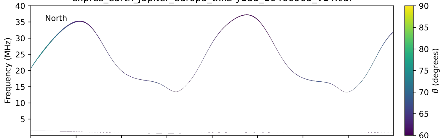
expres_earth_jupiter_europa_txka-y235_20460905_v14.cdf
