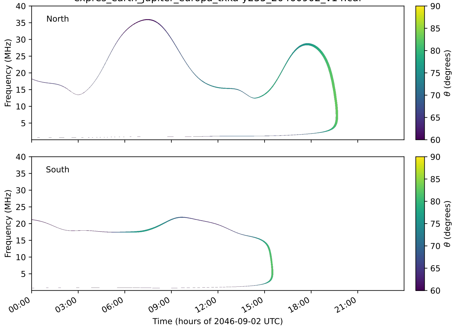
expres_earth_jupiter_europa_txka-y235_20460902_v14.cdf
