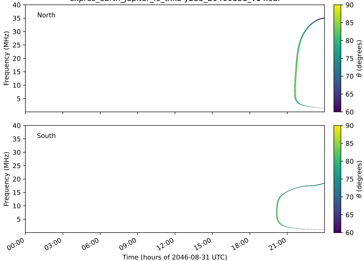
expres_earth_jupiter_io_txka-y235_20460831_v14.cdf
