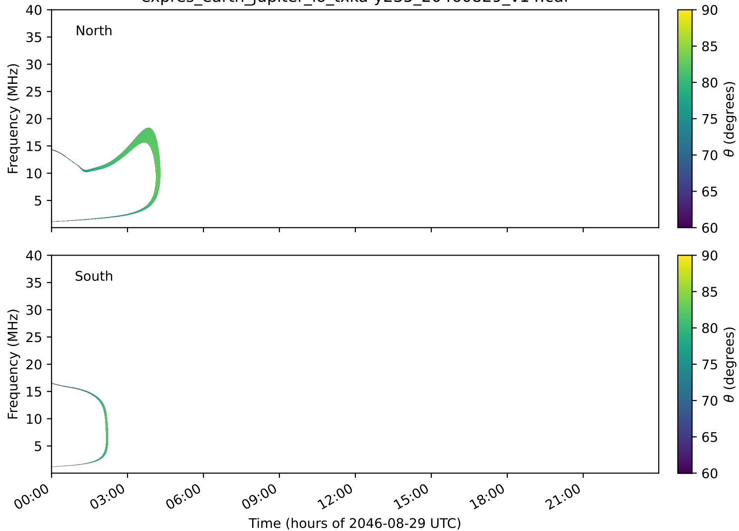
expres_earth_jupiter_io_txka-y235_20460829_v14.cdf
