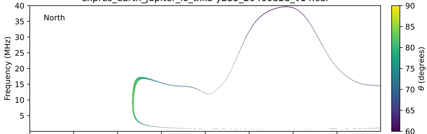
expres_earth_jupiter_io_txka-y235_20460828_v14.cdf
