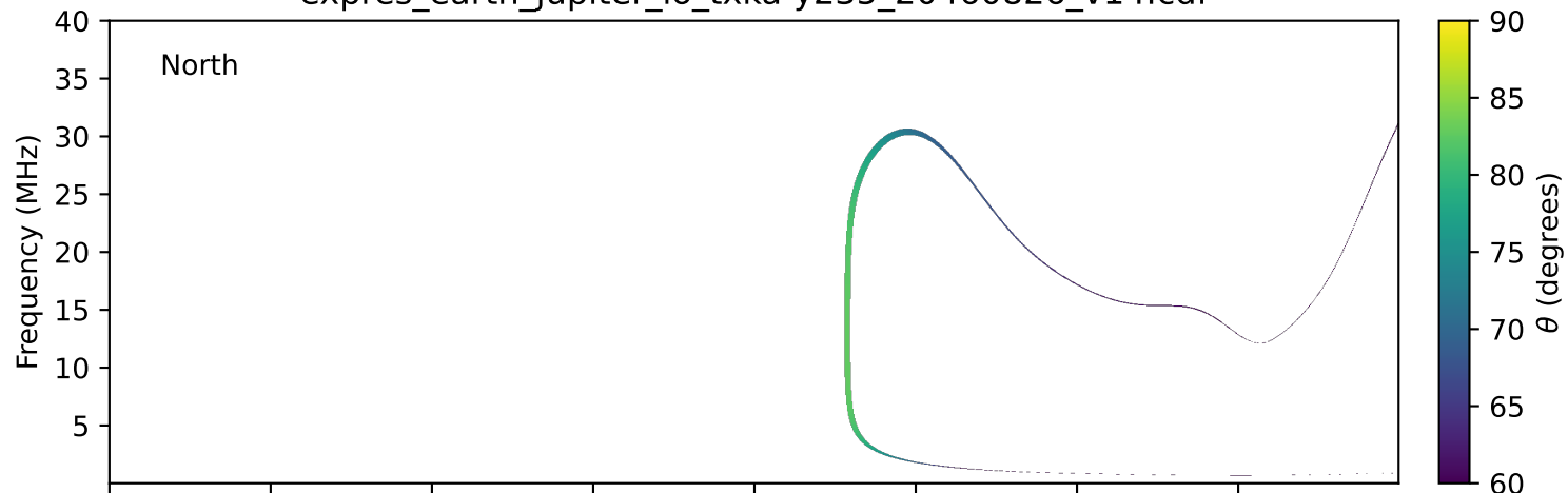
expres_earth_jupiter_io_txka-y235_20460826_v14.cdf
