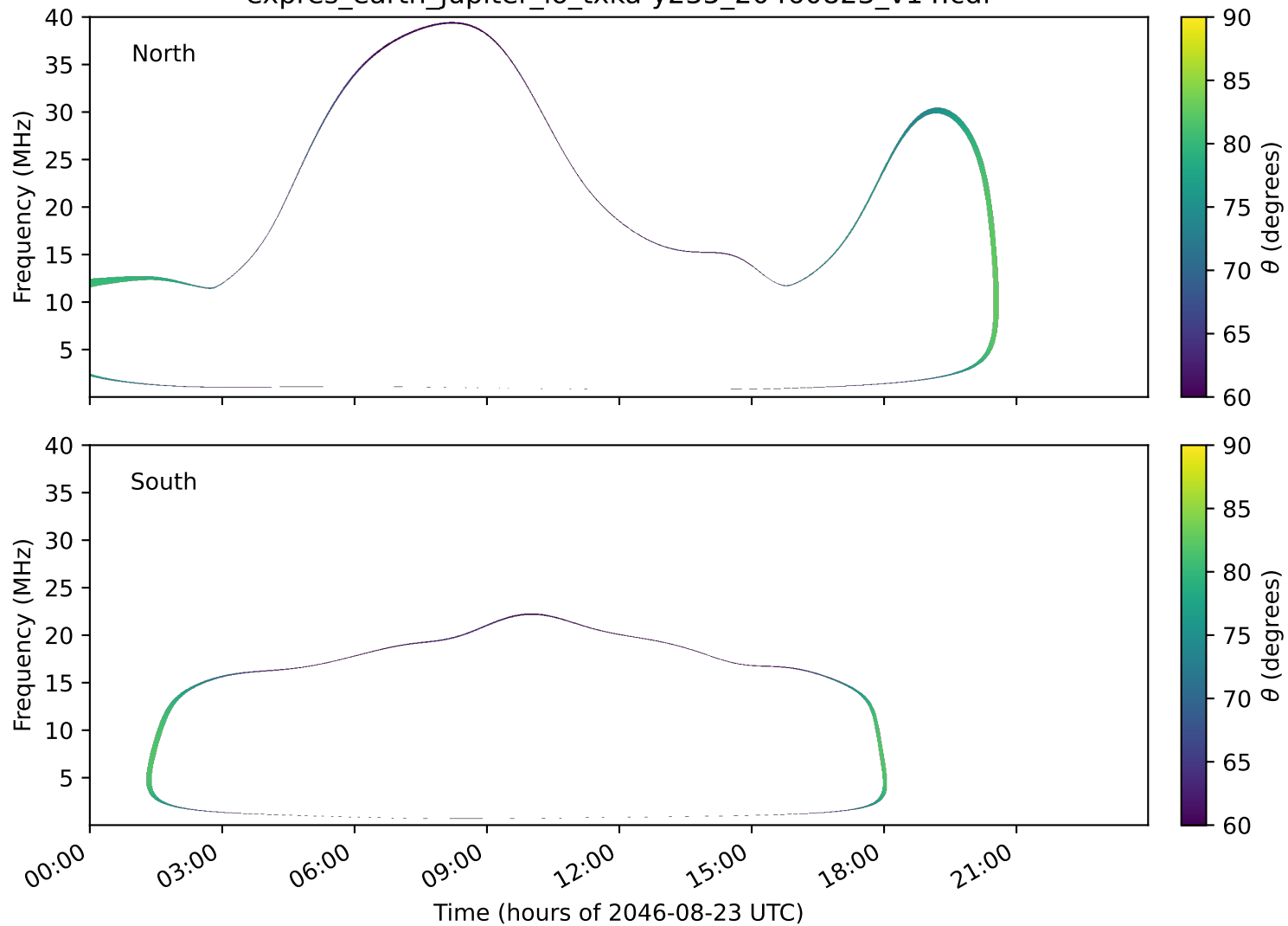
expres_earth_jupiter_io_txka-y235_20460823_v14.cdf
