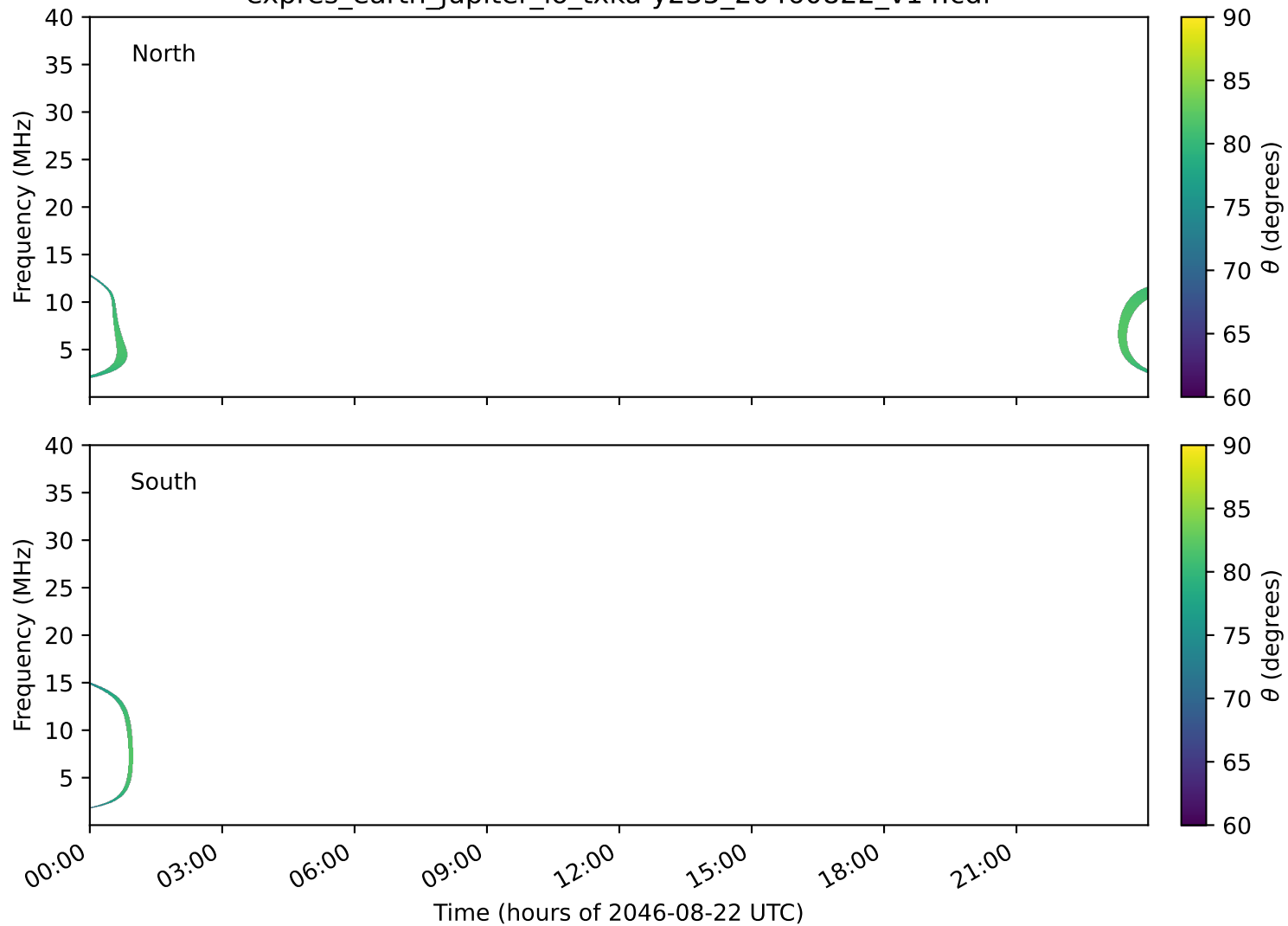
expres_earth_jupiter_io_txka-y235_20460822_v14.cdf
