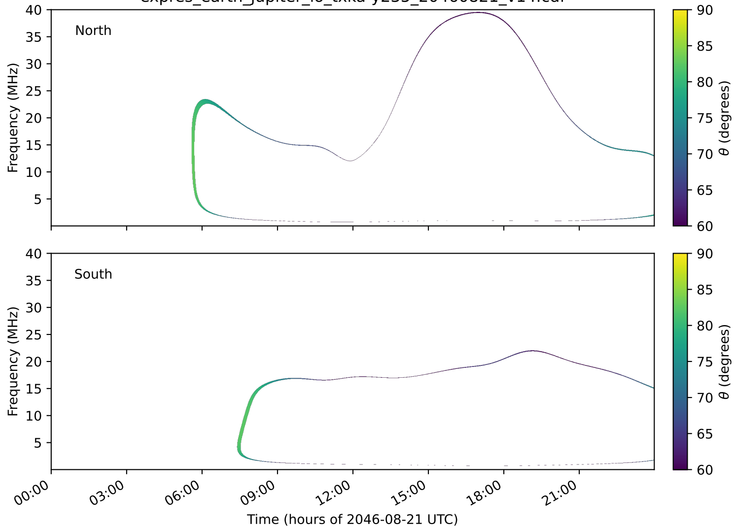
expres_earth_jupiter_io_txka-y235_20460821_v14.cdf
