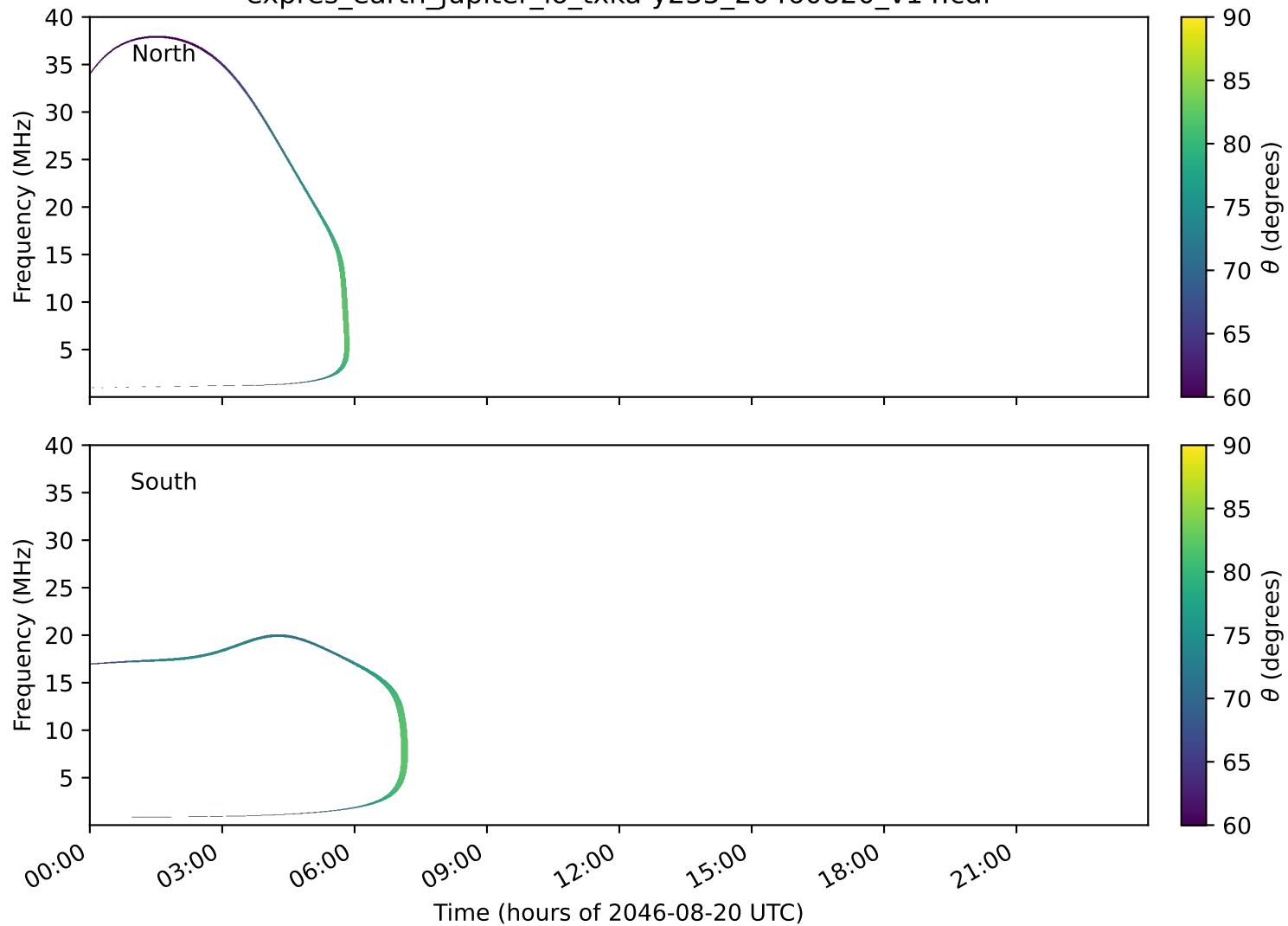
expres_earth_jupiter_io_txka-y235_20460820_v14.cdf
