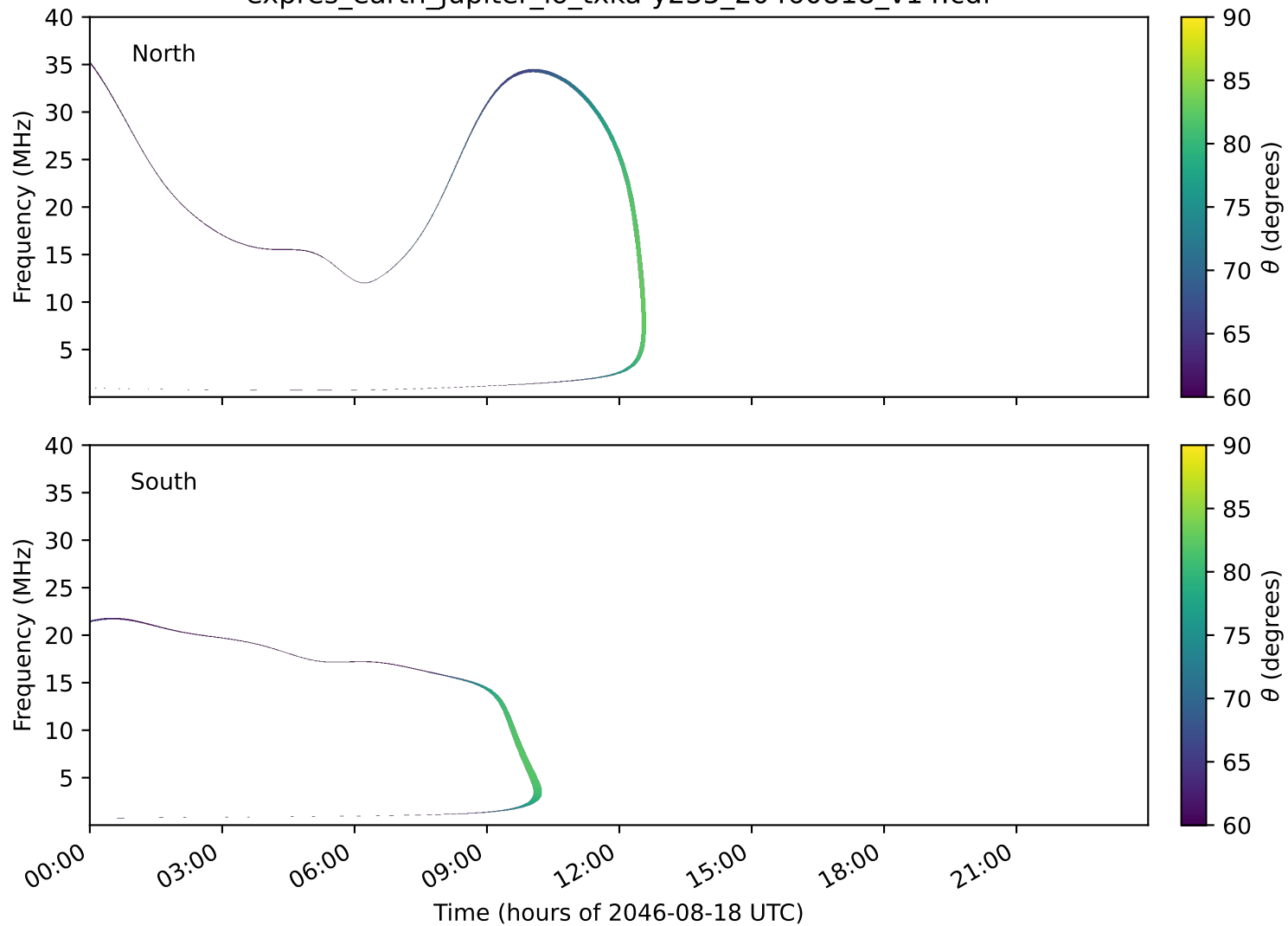
expres_earth_jupiter_io_txka-y235_20460818_v14.cdf
