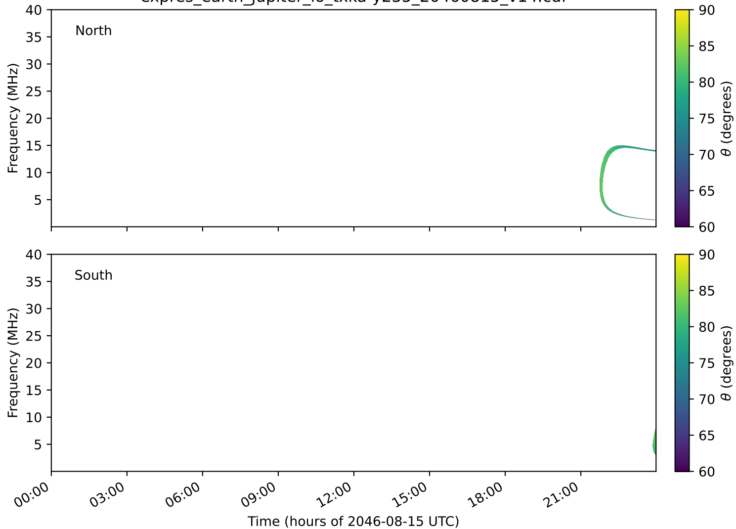
expres_earth_jupiter_io_txka-y235_20460815_v14.cdf
