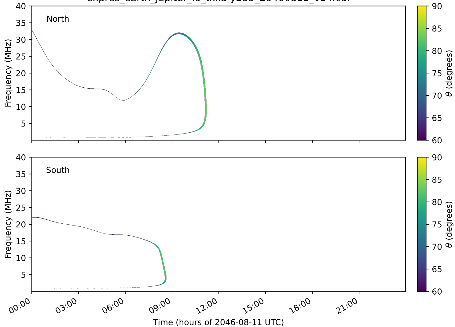
expres_earth_jupiter_io_txka-y235_20460811_v14.cdf
