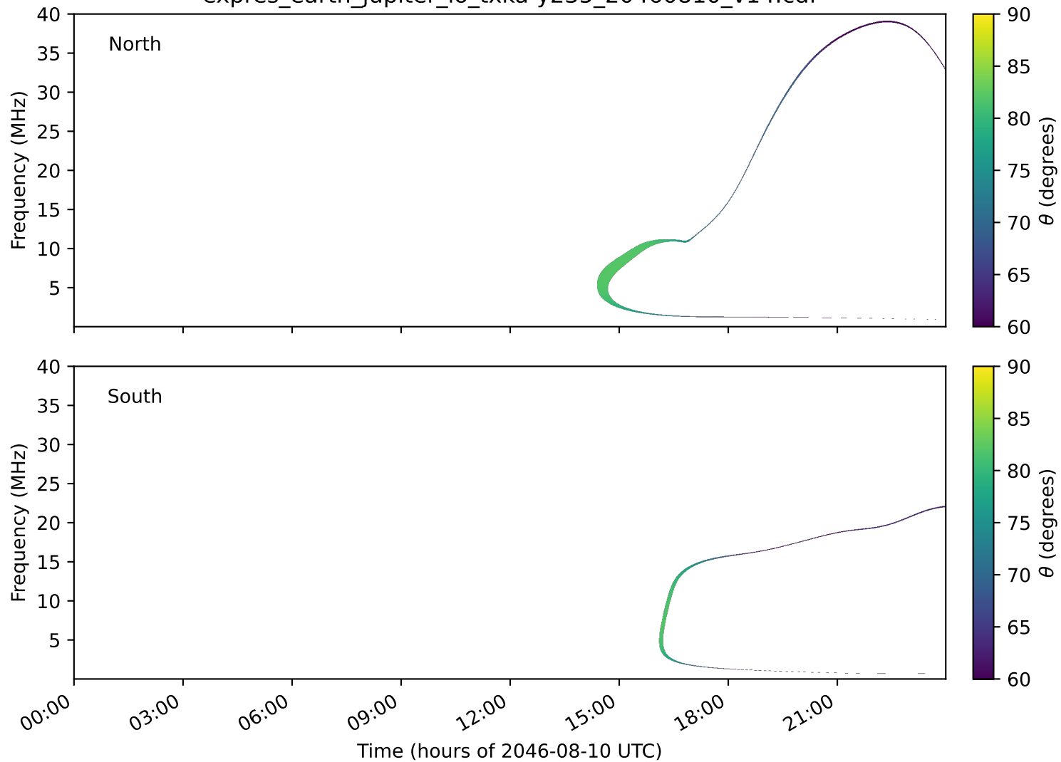
expres_earth_jupiter_io_txka-y235_20460810_v14.cdf
