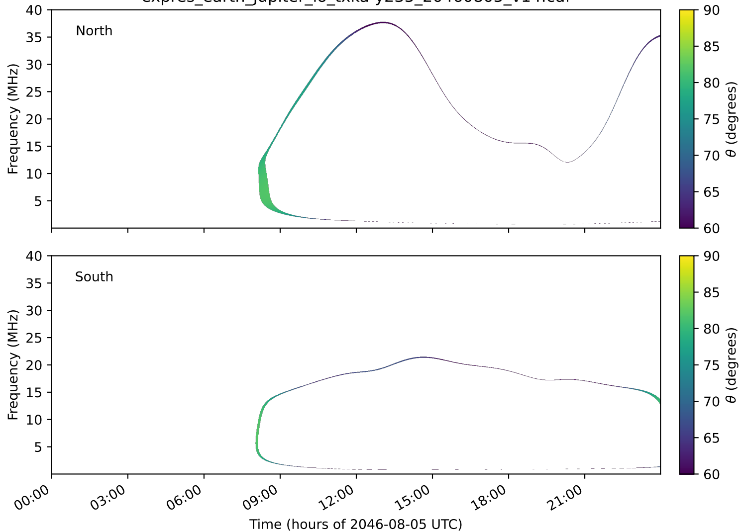
expres_earth_jupiter_io_txka-y235_20460805_v14.cdf
