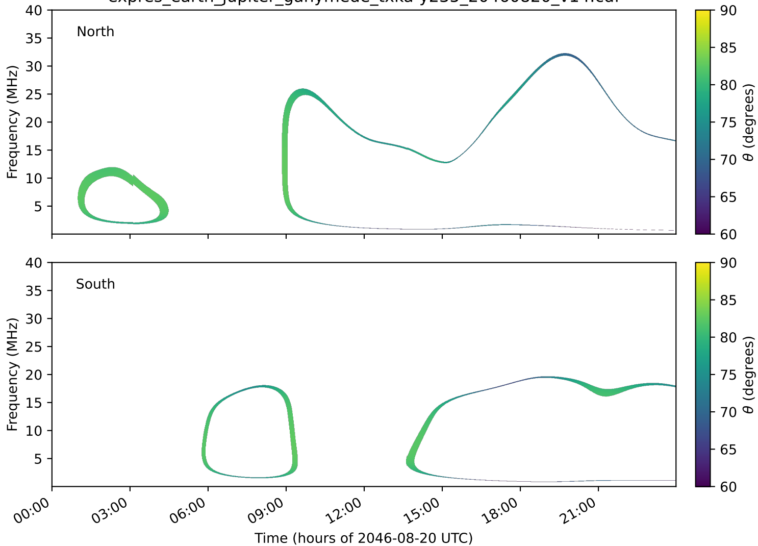
expres_earth_jupiter_ganymede_txka-y235_20460820_v14.cdf
