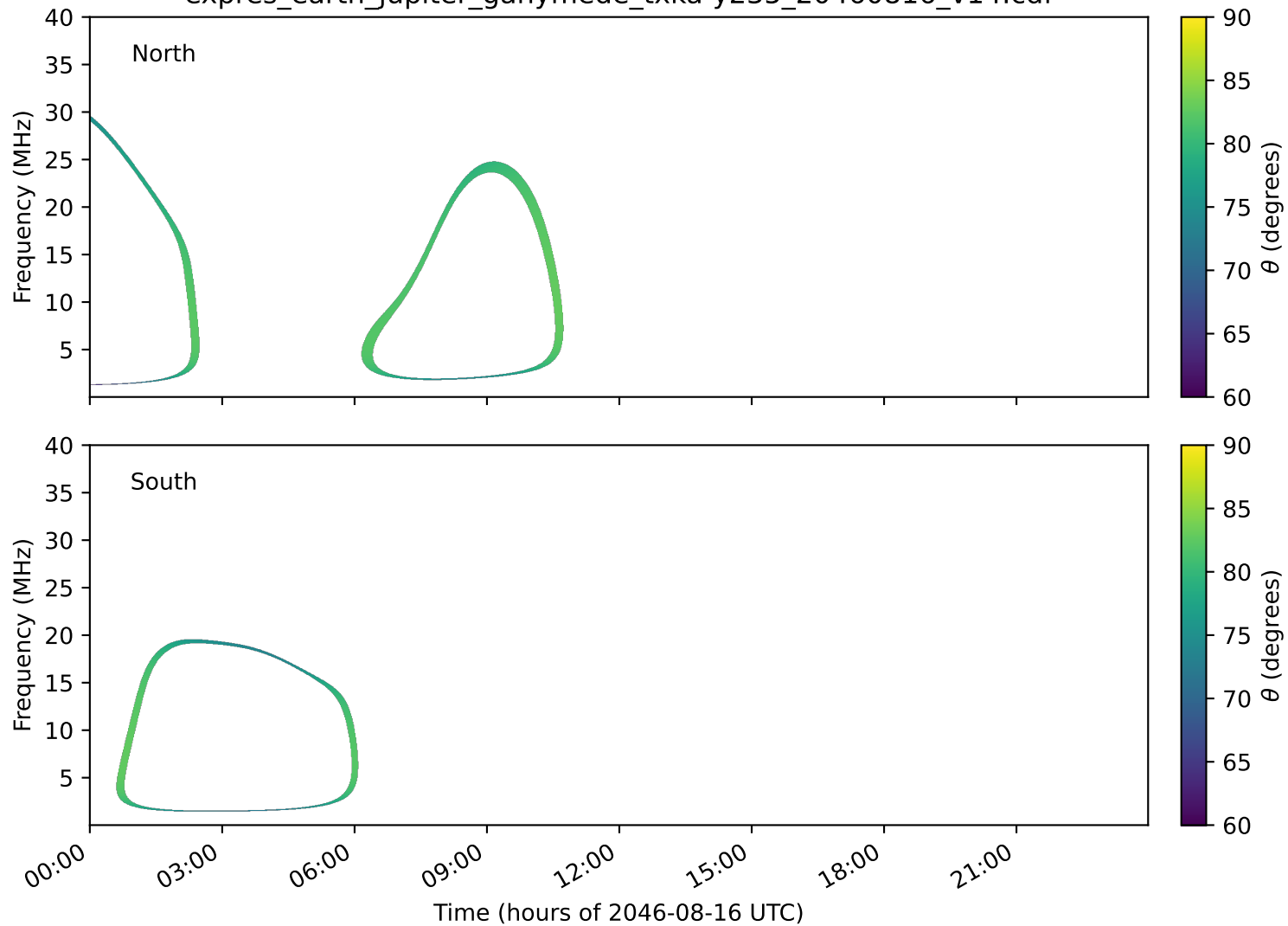
expres_earth_jupiter_ganymede_txka-y235_20460816_v14.cdf
