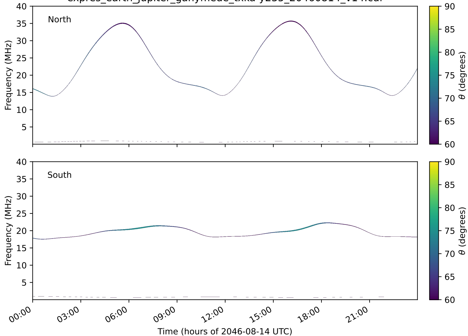
expres_earth_jupiter_ganymede_txka-y235_20460814_v14.cdf
