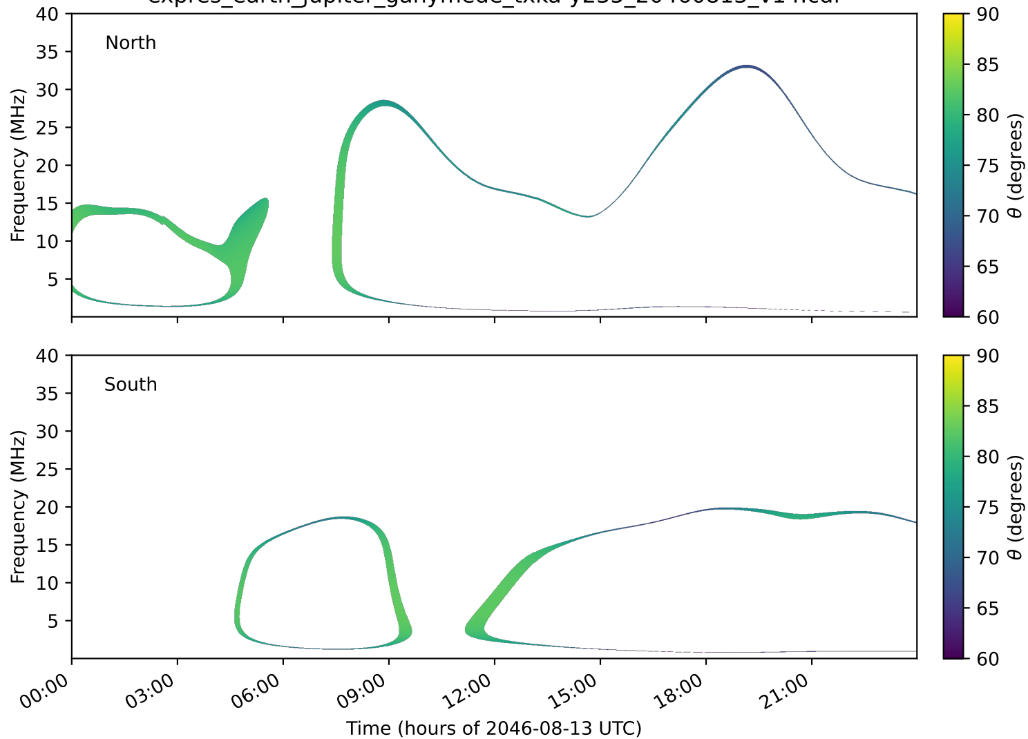
expres_earth_jupiter_ganymede_txka-y235_20460813_v14.cdf
