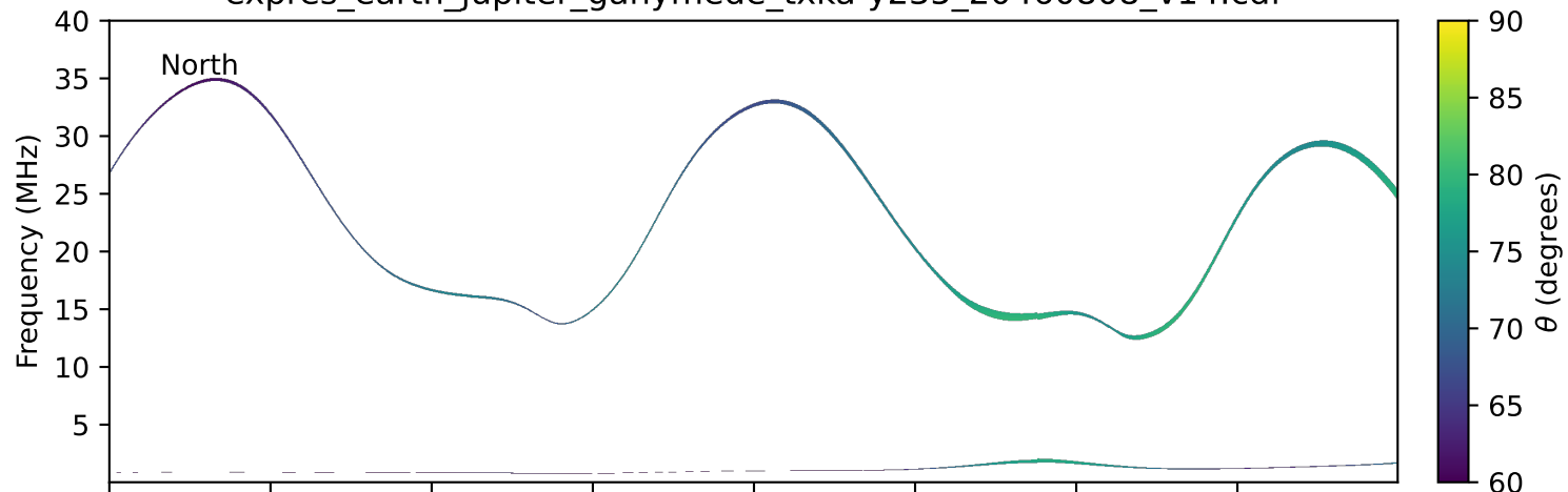
expres_earth_jupiter_ganymede_txka-y235_20460808_v14.cdf
