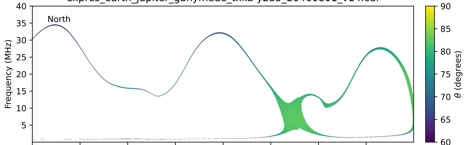
expres_earth_jupiter_ganymede_txka-y235_20460801_v14.cdf
