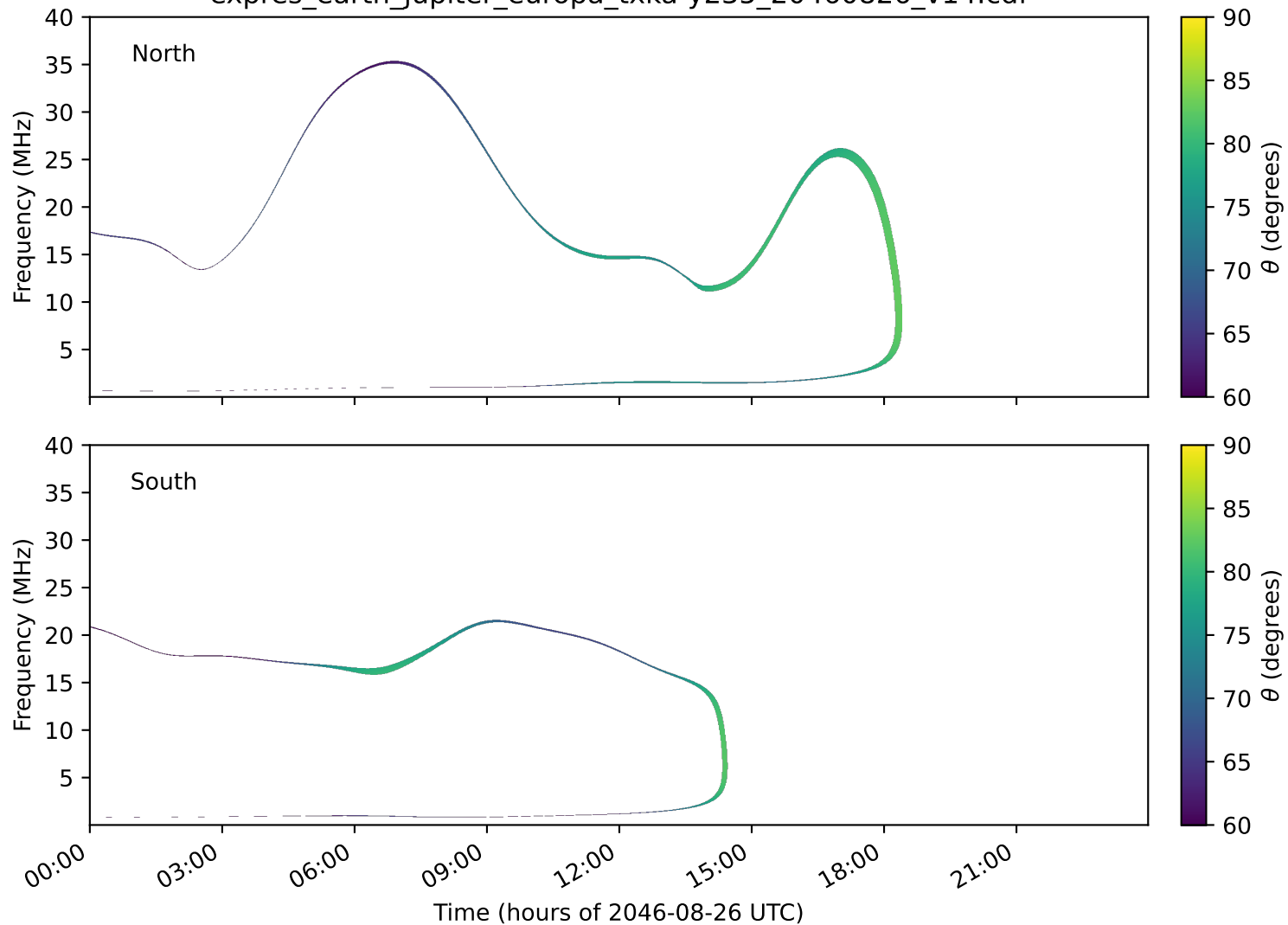
expres_earth_jupiter_europa_txka-y235_20460826_v14.cdf
