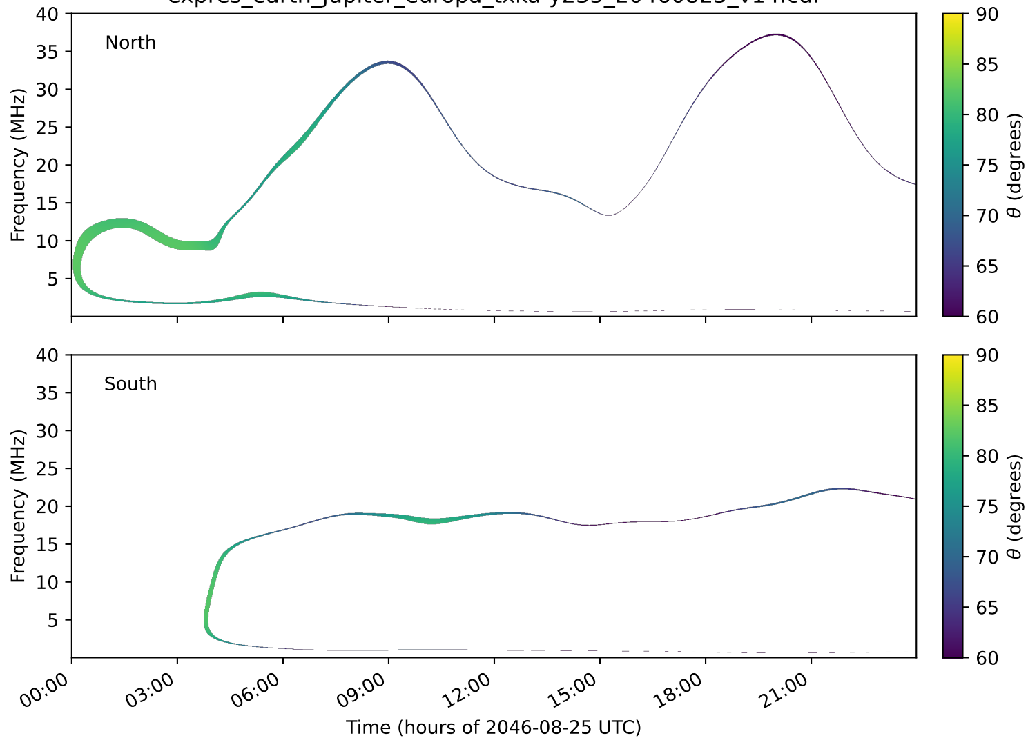
expres_earth_jupiter_europa_txka-y235_20460825_v14.cdf
