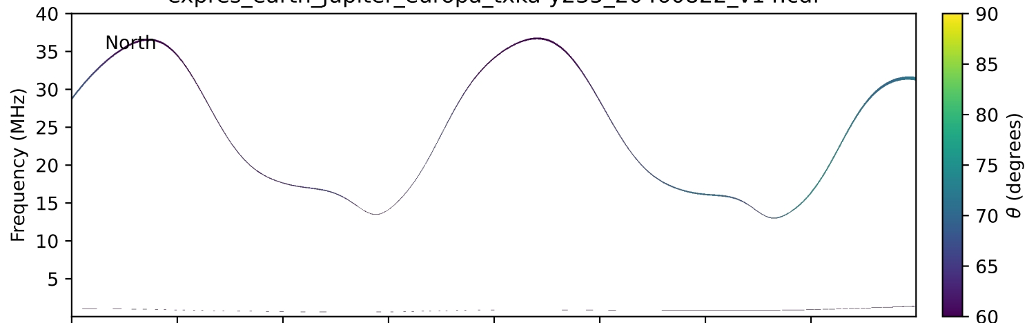
expres_earth_jupiter_europa_txka-y235_20460822_v14.cdf
