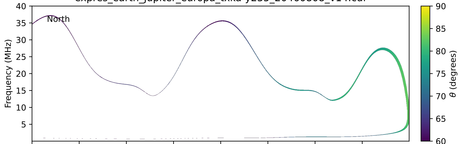
expres_earth_jupiter_europa_txka-y235_20460808_v14.cdf
