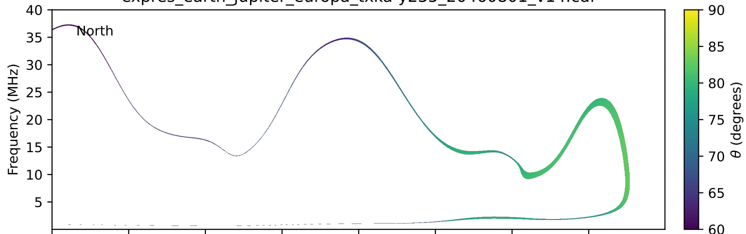
expres_earth_jupiter_europa_txka-y235_20460801_v14.cdf
