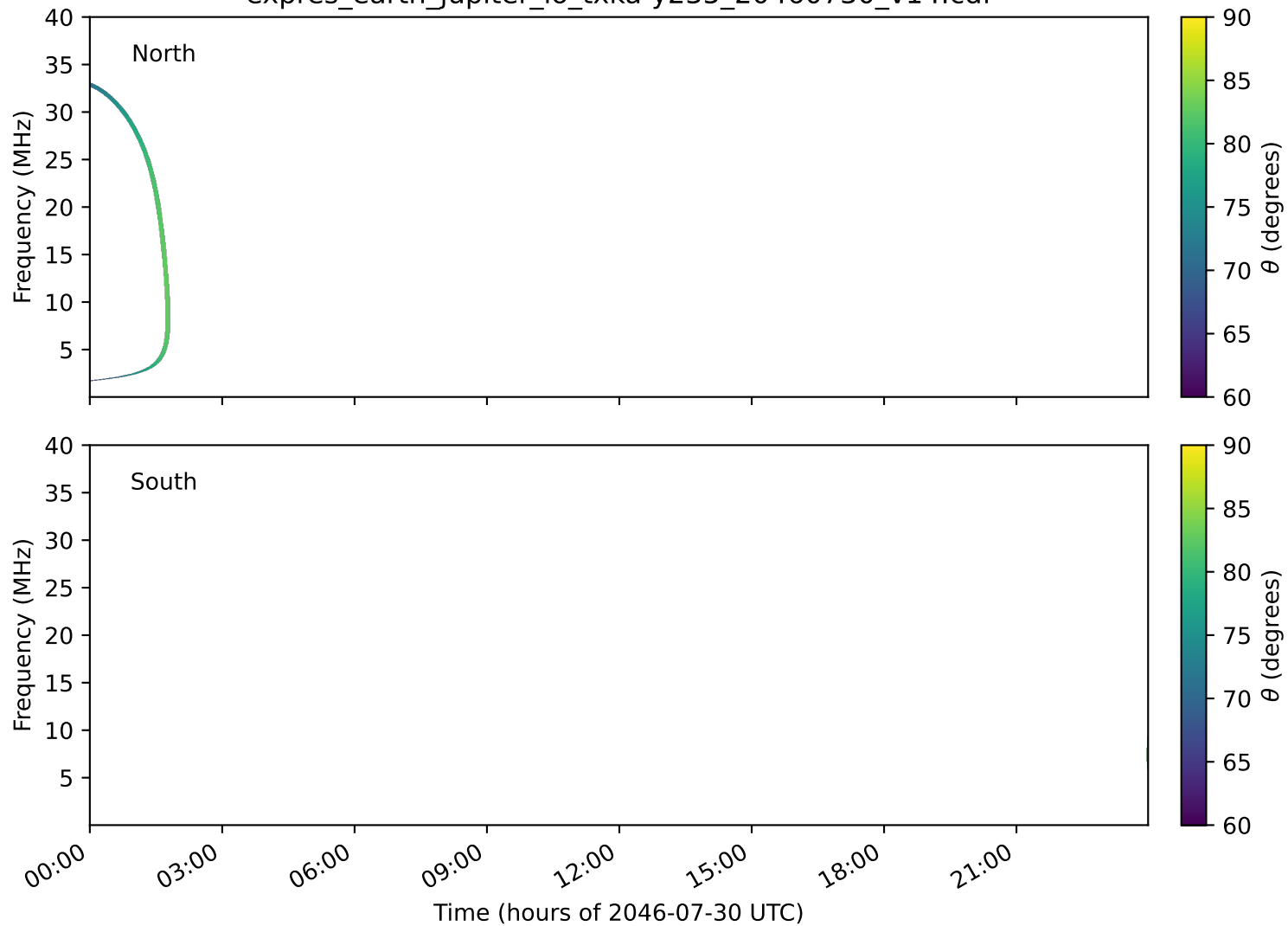
expres_earth_jupiter_io_txka-y235_20460730_v14.cdf
