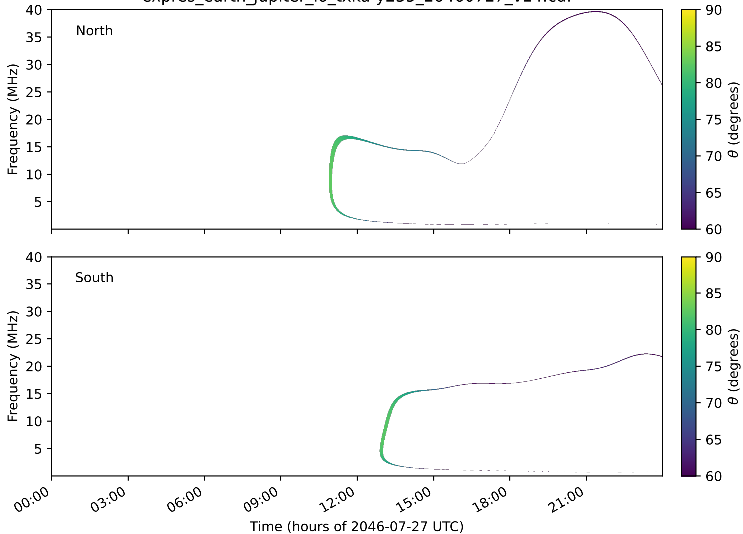
expres_earth_jupiter_io_txka-y235_20460727_v14.cdf
