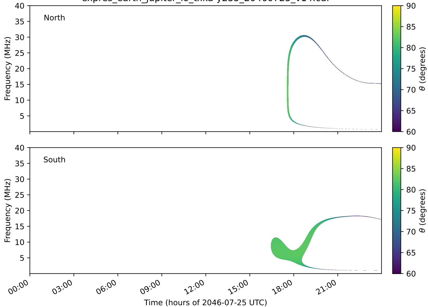
expres_earth_jupiter_io_txka-y235_20460725_v14.cdf
