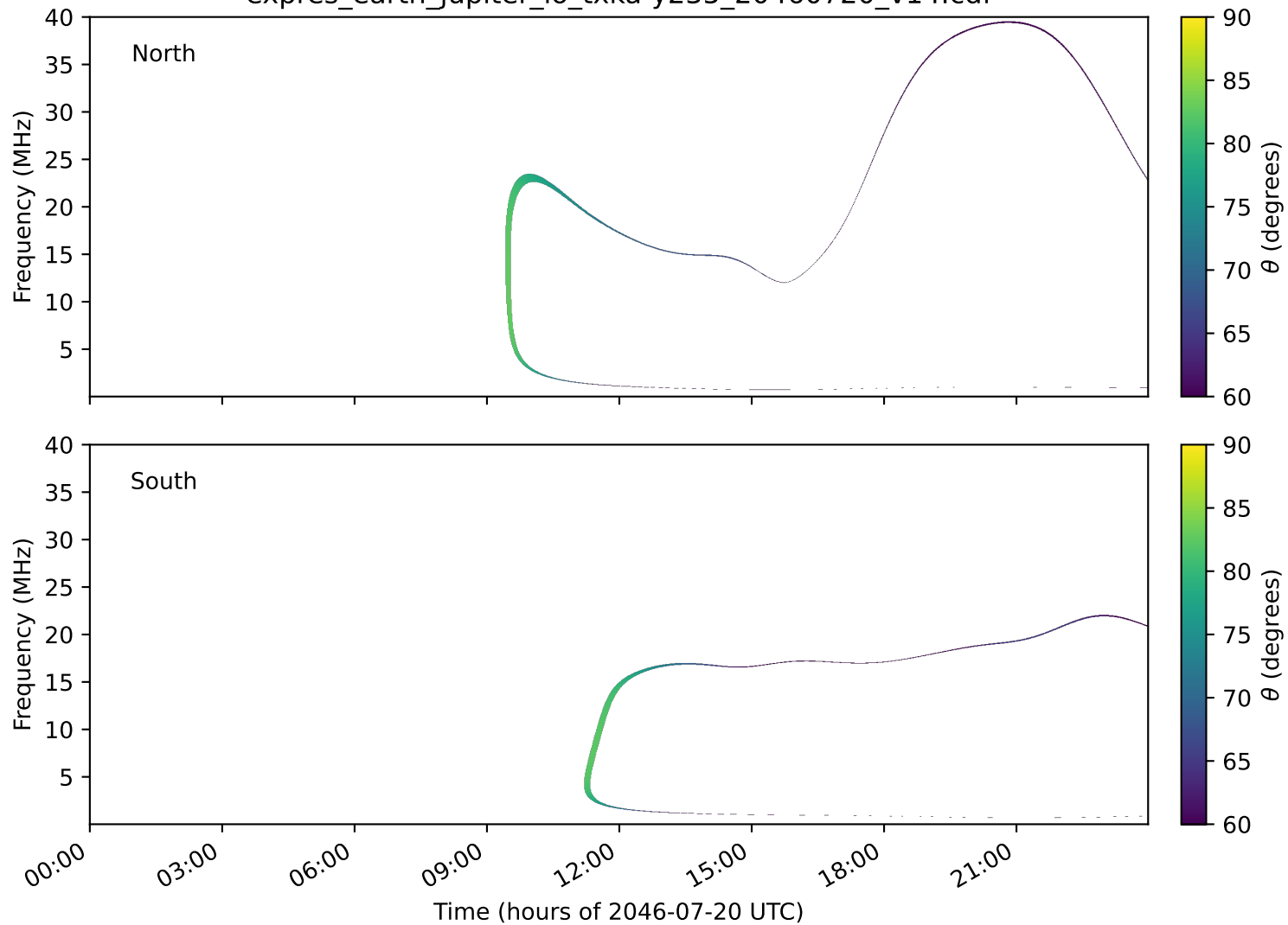
expres_earth_jupiter_io_txka-y235_20460720_v14.cdf
