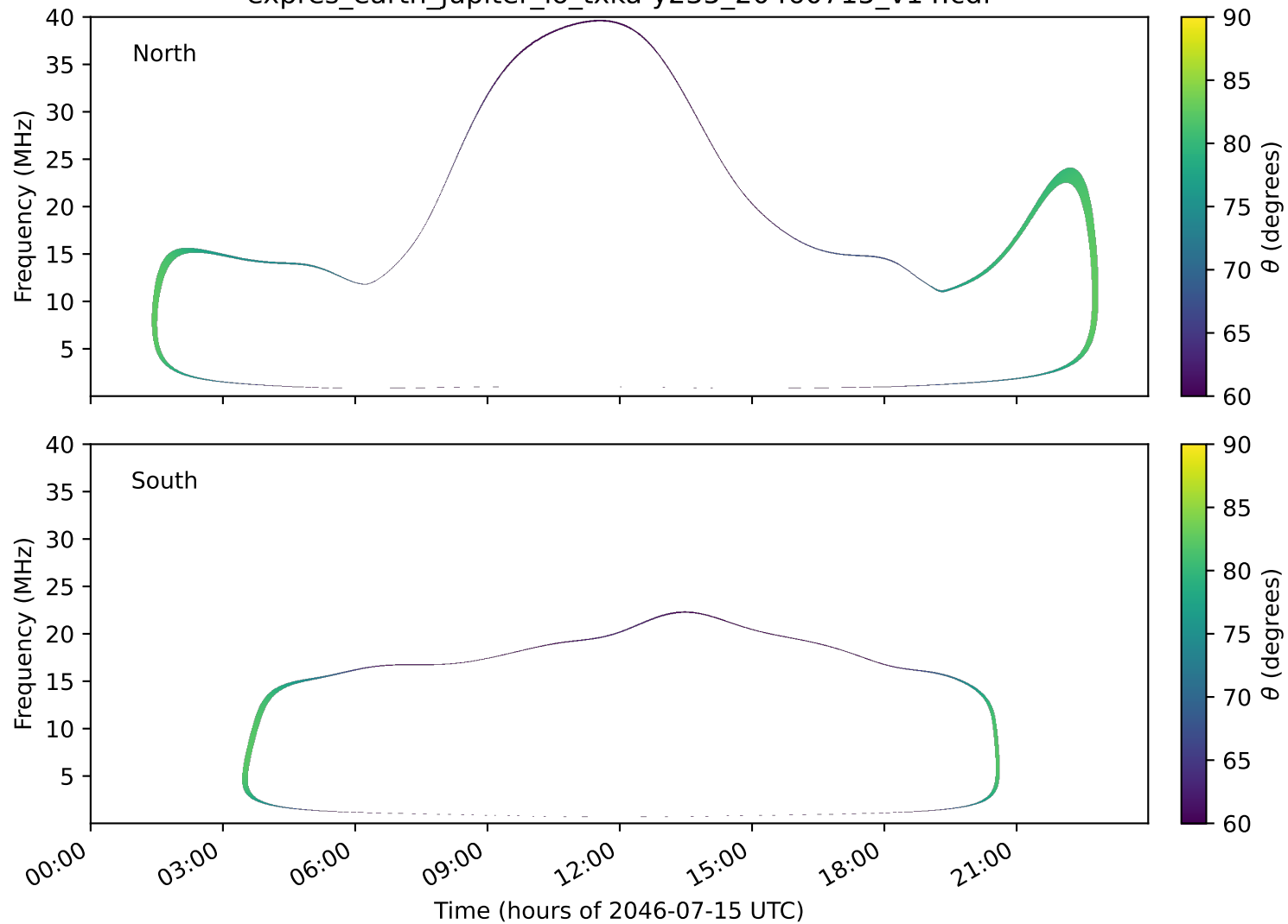
expres_earth_jupiter_io_txka-y235_20460715_v14.cdf
