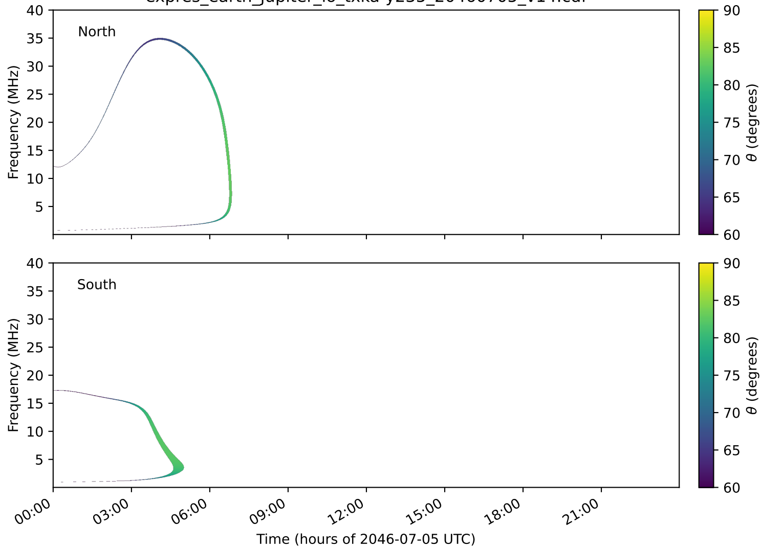
expres_earth_jupiter_io_txka-y235_20460705_v14.cdf
