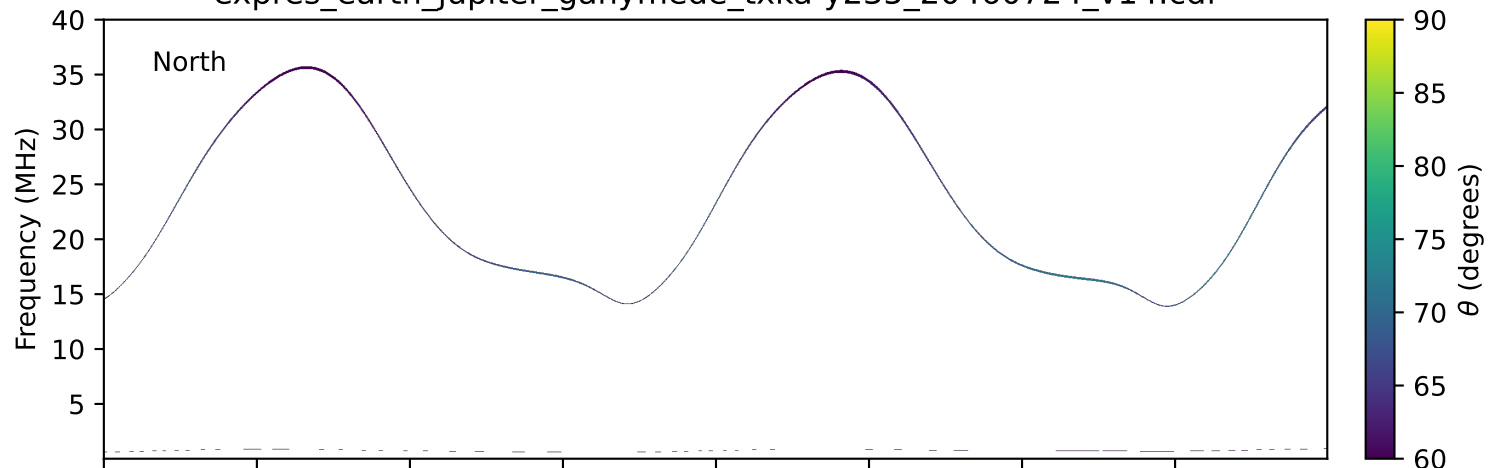
expres_earth_jupiter_ganymede_txka-y235_20460724_v14.cdf
