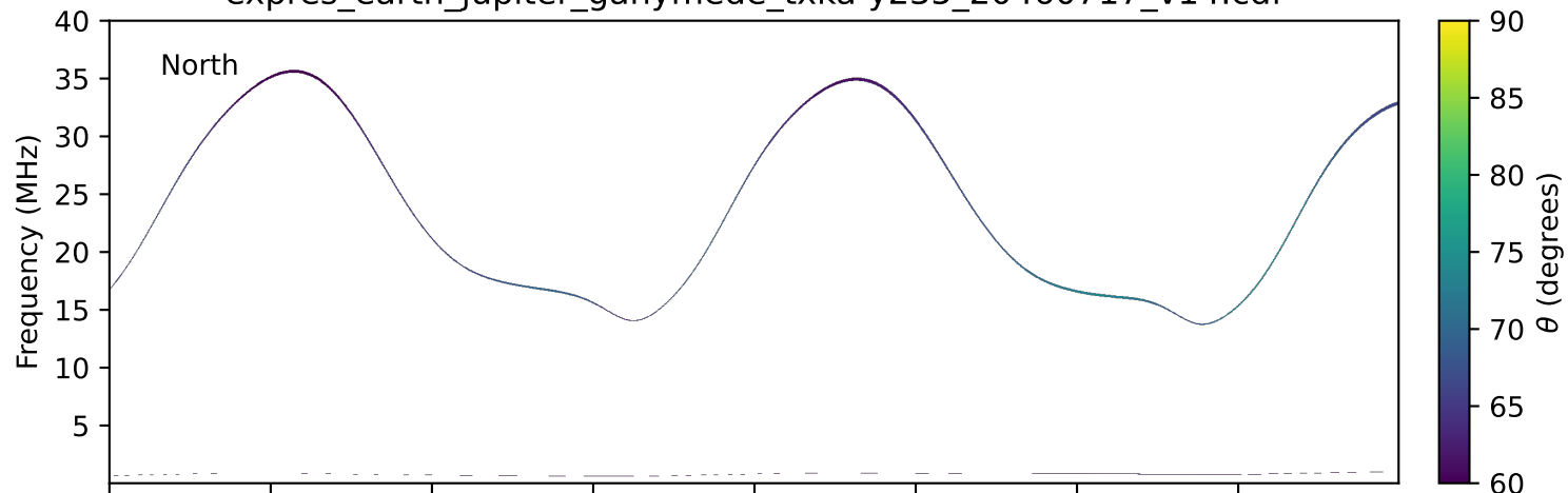
expres_earth_jupiter_ganymede_txka-y235_20460717_v14.cdf
