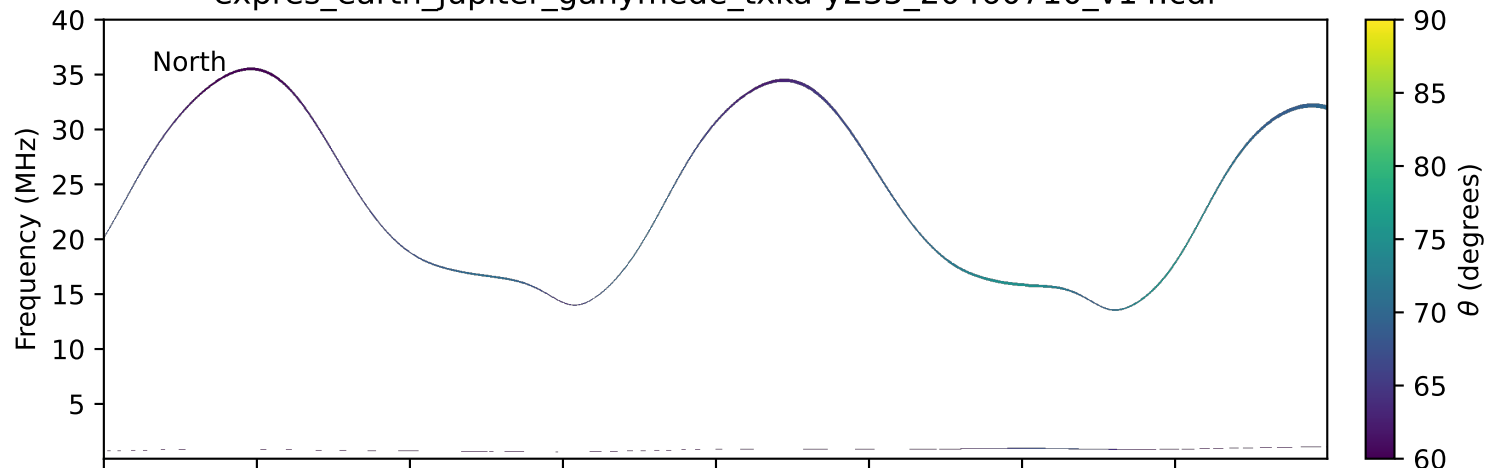
expres_earth_jupiter_ganymede_txka-y235_20460710_v14.cdf
