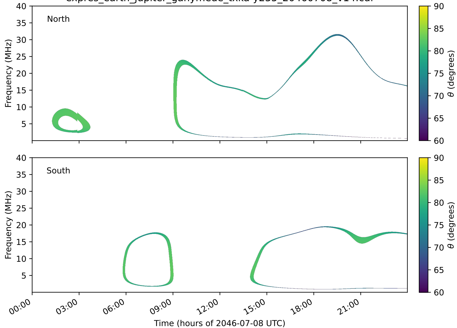
expres_earth_jupiter_ganymede_txka-y235_20460708_v14.cdf
