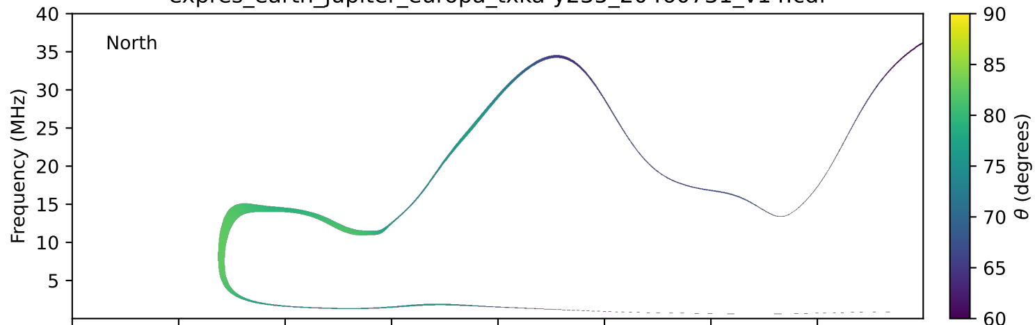
expres_earth_jupiter_europa_txka-y235_20460731_v14.cdf
