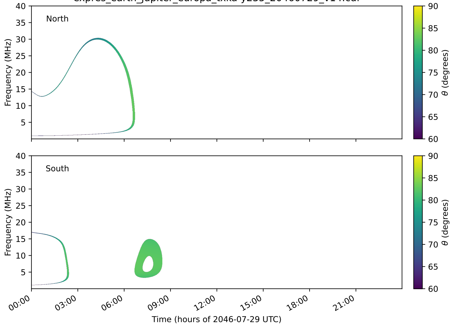
expres_earth_jupiter_europa_txka-y235_20460729_v14.cdf
